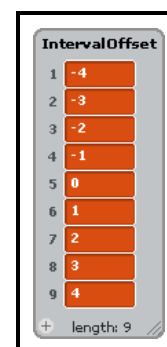
Figure 5b. Interval list for use with the “random walk” algorithm.
